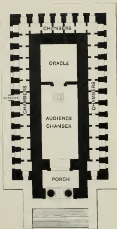
GROUND PLAN.
